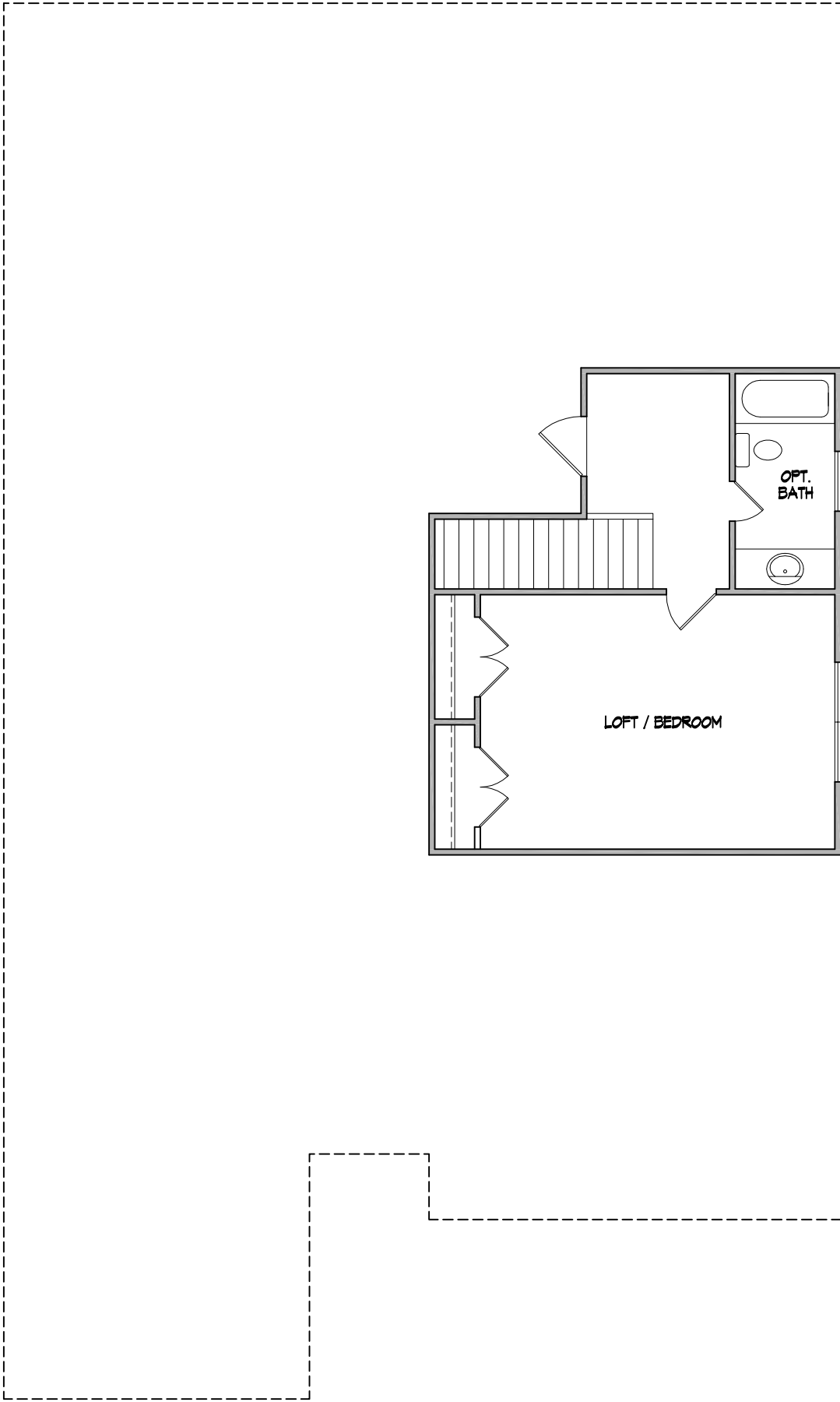
MODEL NANTUCKET w/ LOFT - SECOND FLOOR
