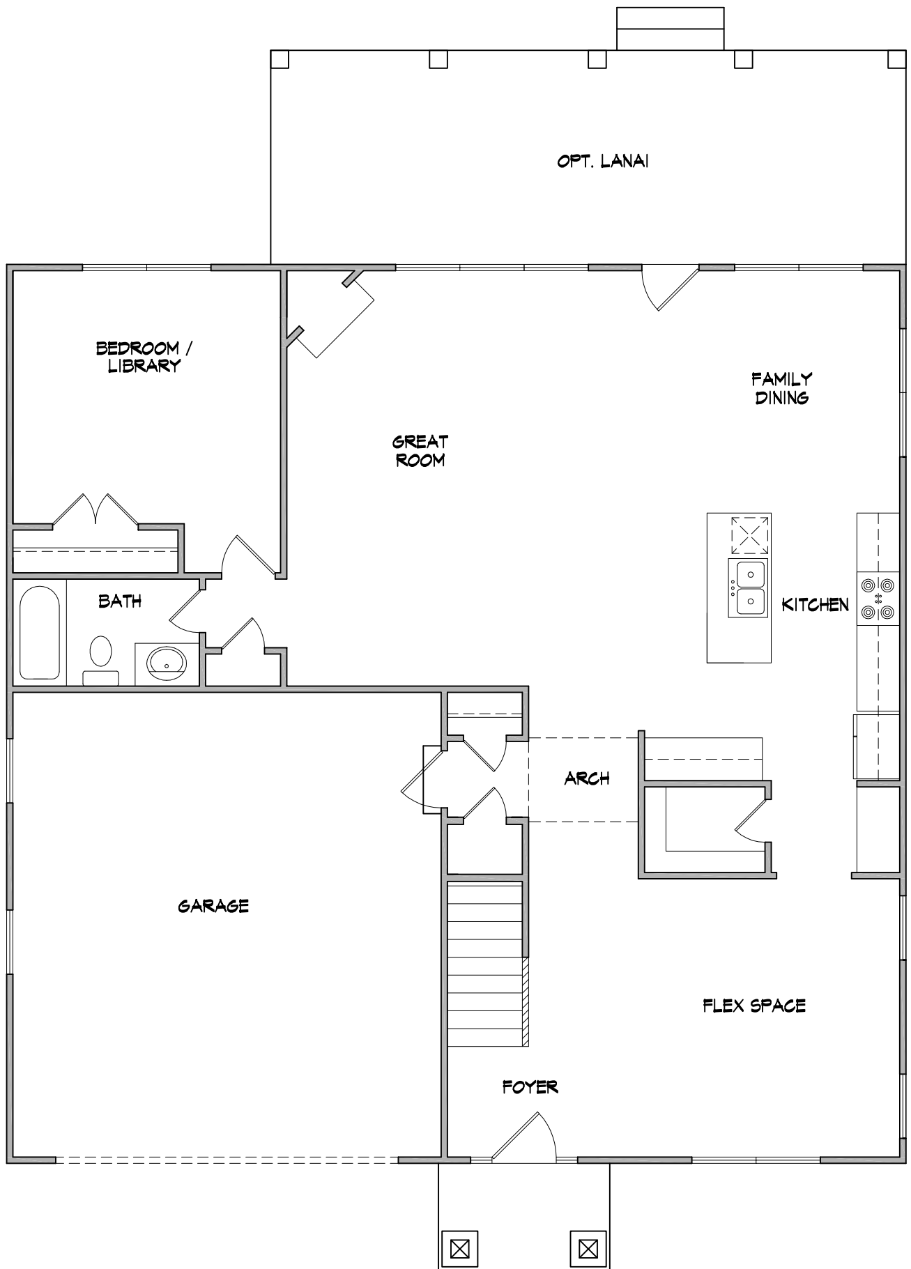
MODEL SAVANNAH - FIRST FLOOR
